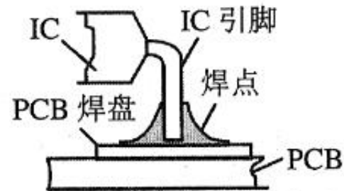
(c) I形引脚
